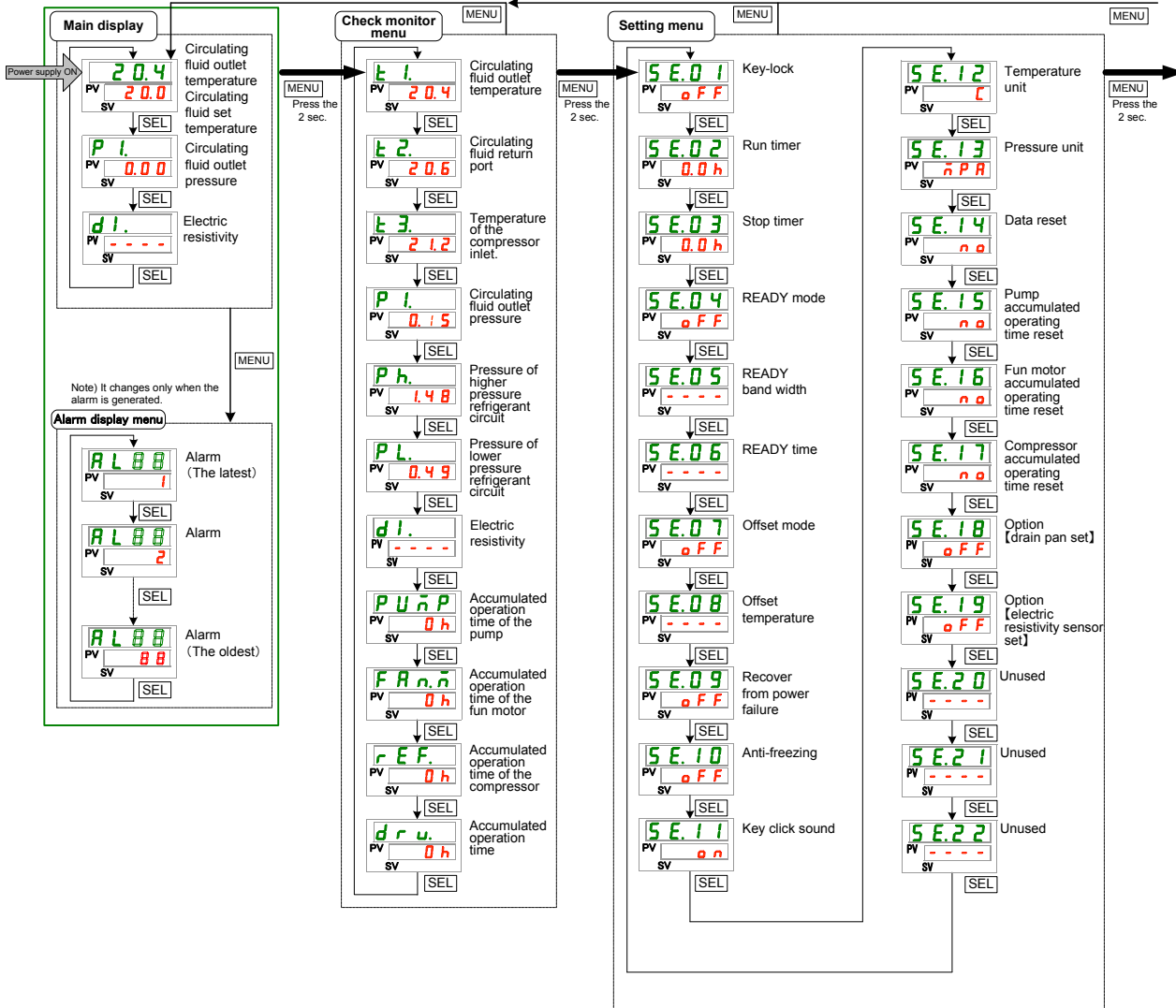
Fig 1.3-1 Key operation (1/2)
