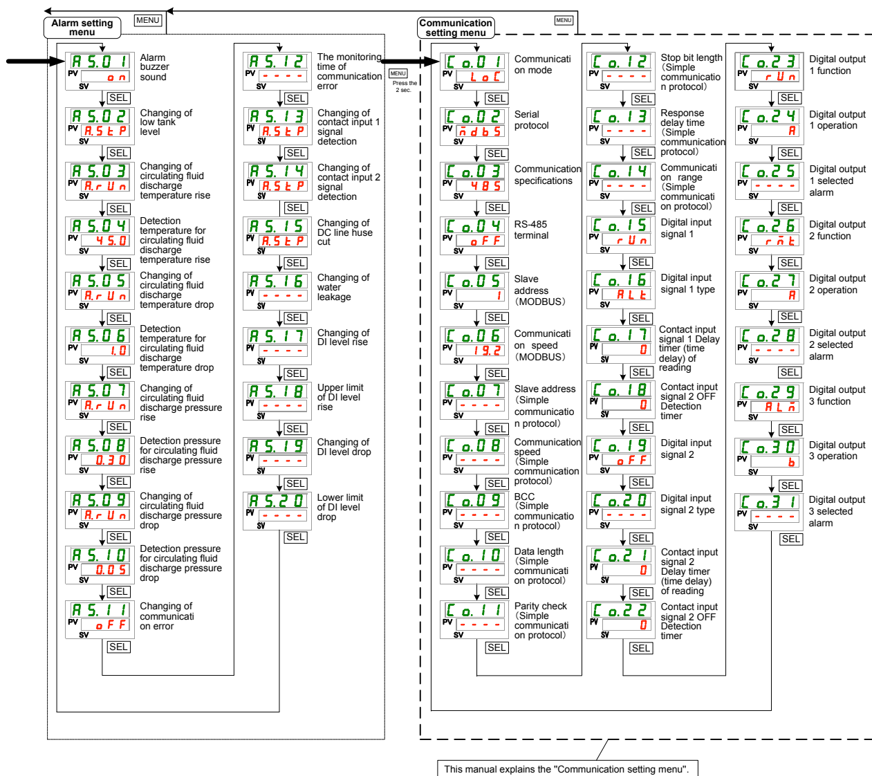
Fig 1.3-2 Key operation (2/2)
