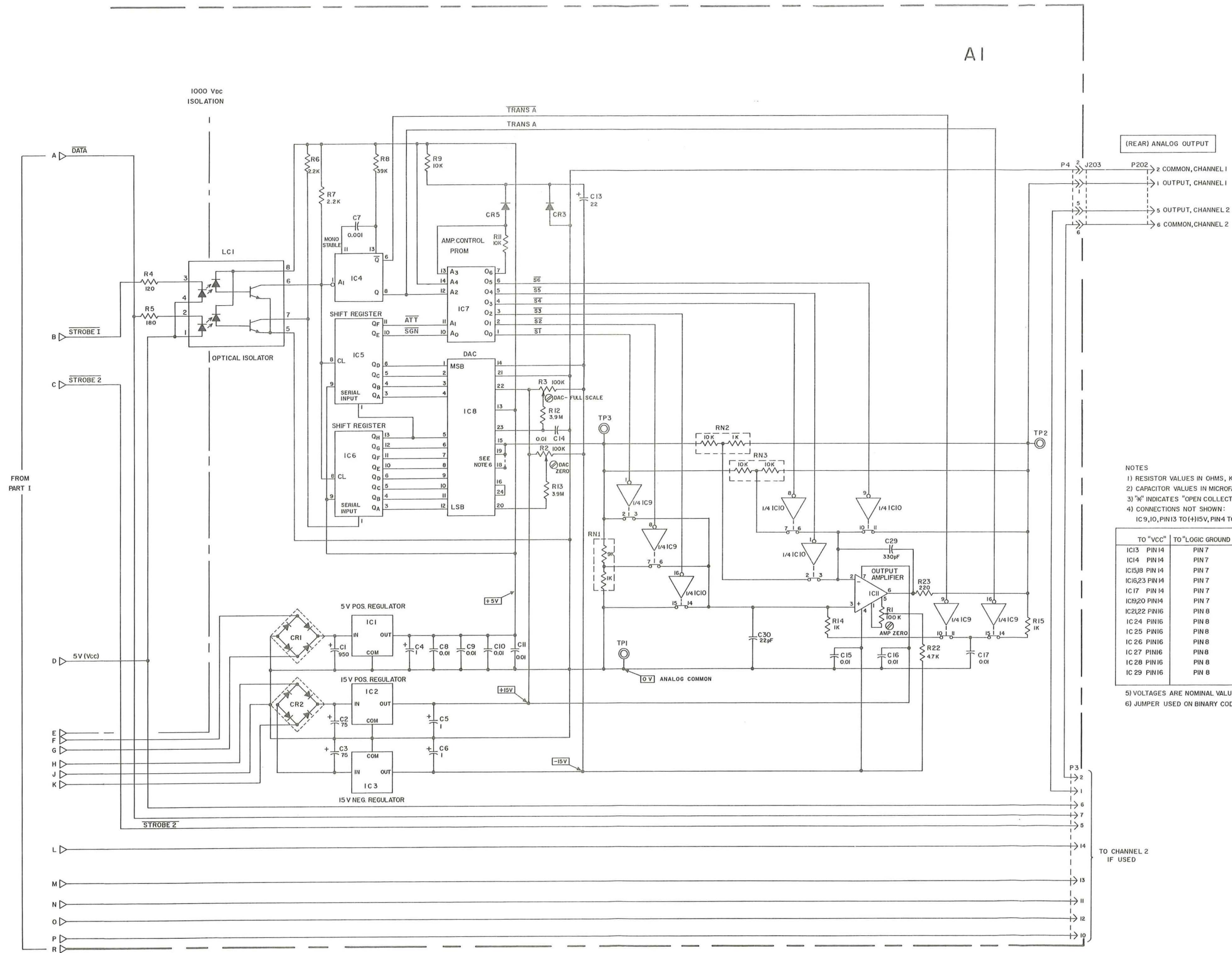
FIG. 5-4 SCHEMATIC DIAGRAM—PART II, SN 488 1/4 SERIES.
