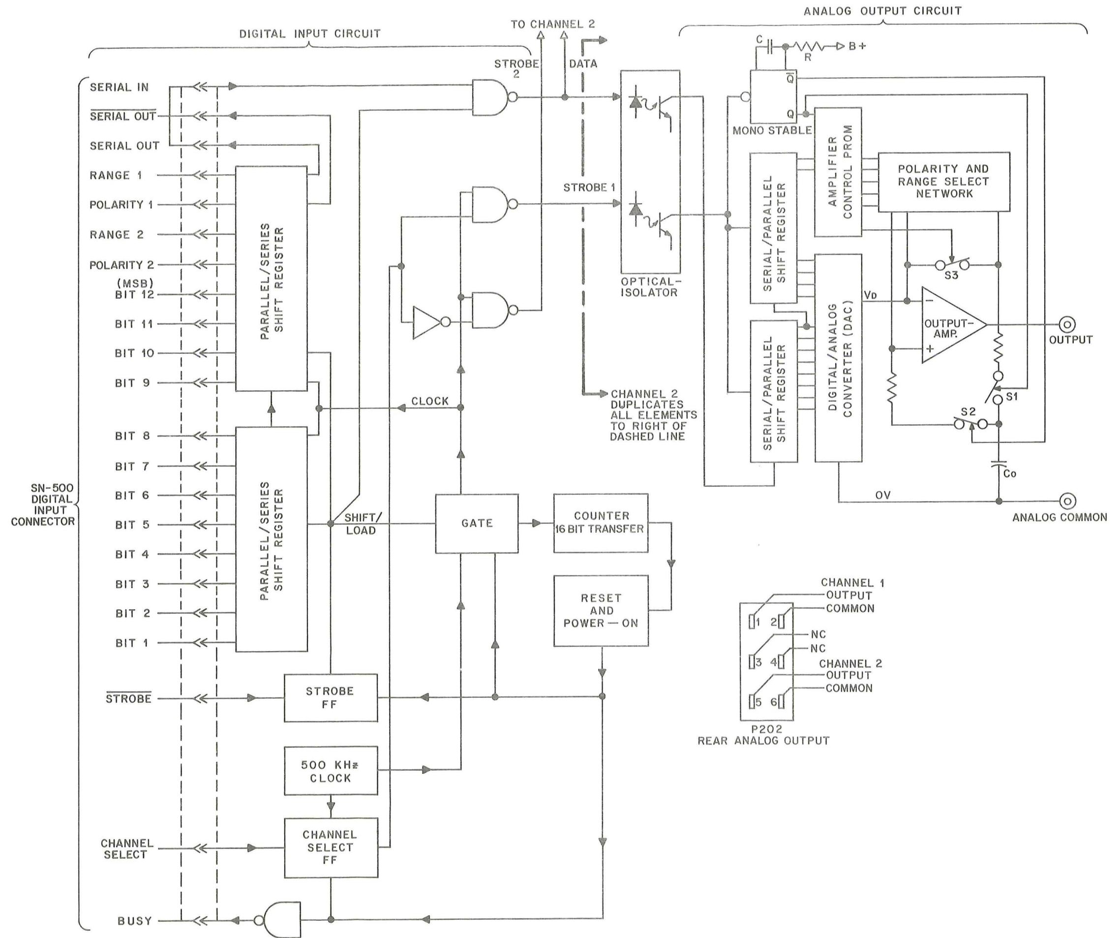
FIG. 4-2 BLOCK DIAGRAM, KEPCO SERIES 500 PROGRAMMER
