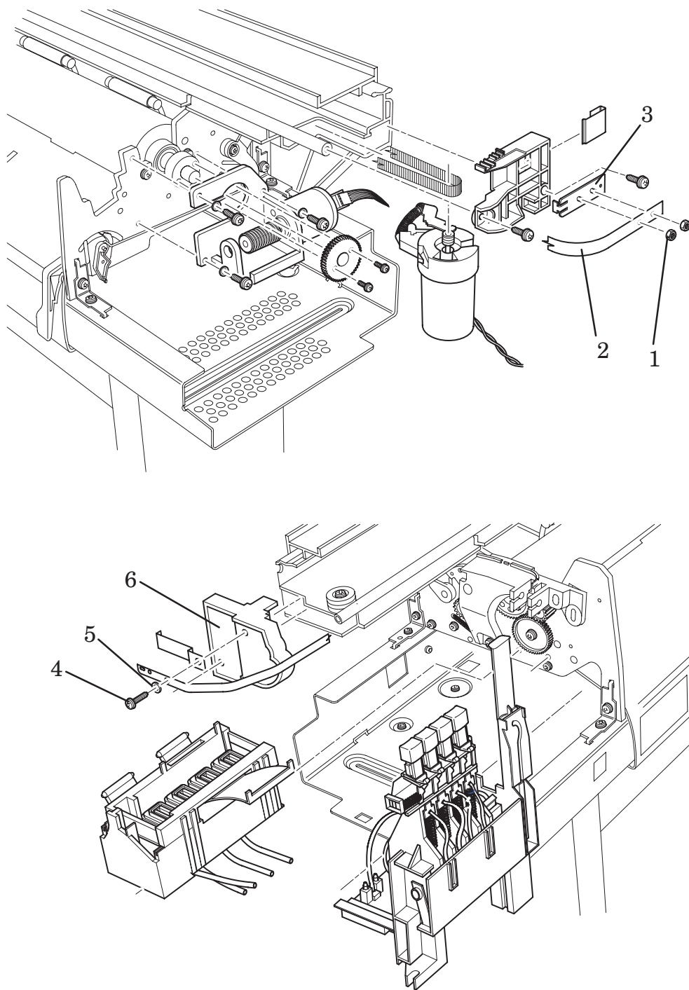
Figure 4: Encoder Strip
