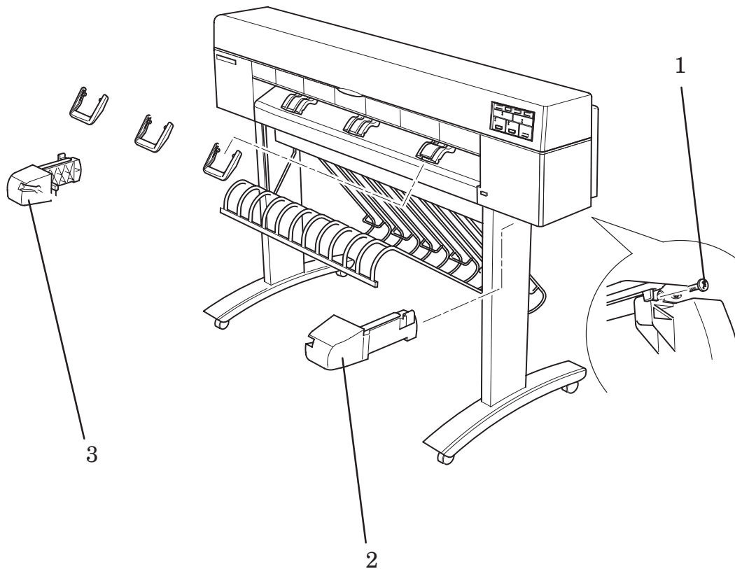
Figure 1: Rollfeed Assembly
