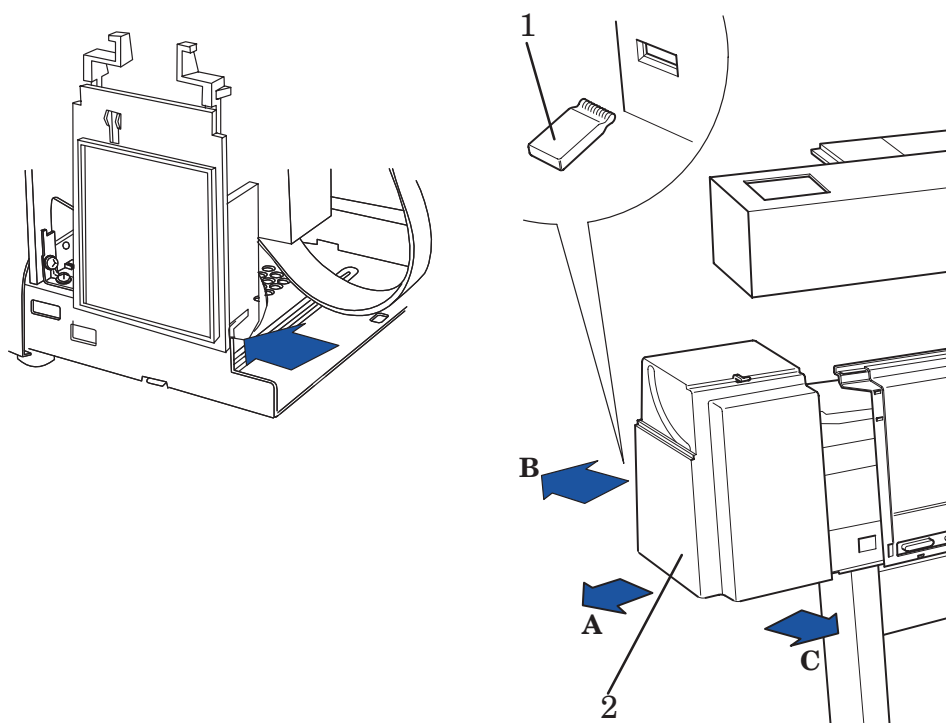
Figure 2: Right End-Cover
