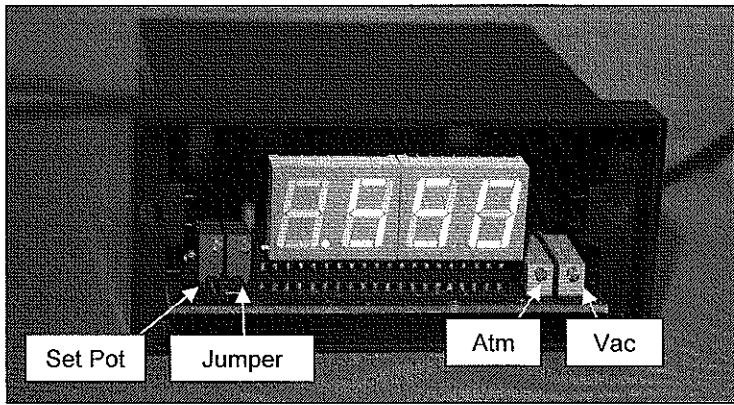
Model 200P with red lens removed
