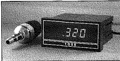
Model 801W and 801W/2c (Varian or Hastings pattern, panel mounting)
